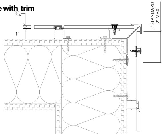
EASY MEG Vertical Standoff Clip Detail Set for Complete Details*
