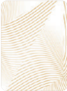
5798 Snow Haze
